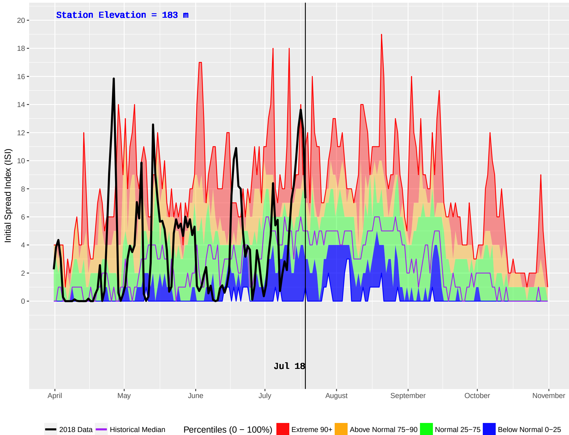
MESACHIE 2 (934) : Historical (2006–2016) and Current (2018) Daily Initial Spread Index (ISI)
