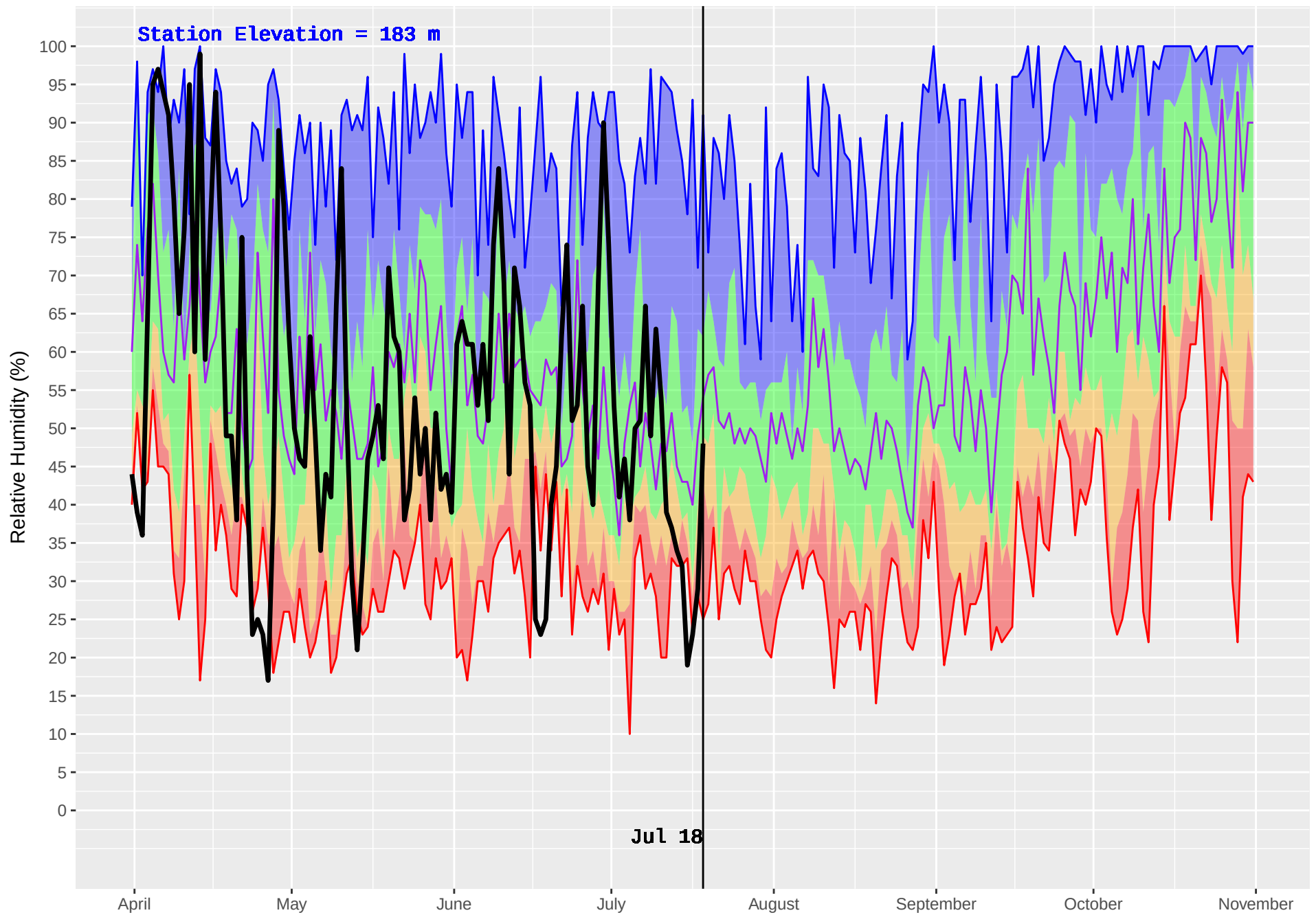
MESACHIE 2 (934) : Historical (2006–2016) and Current (2018) Daily Relative Humidity
