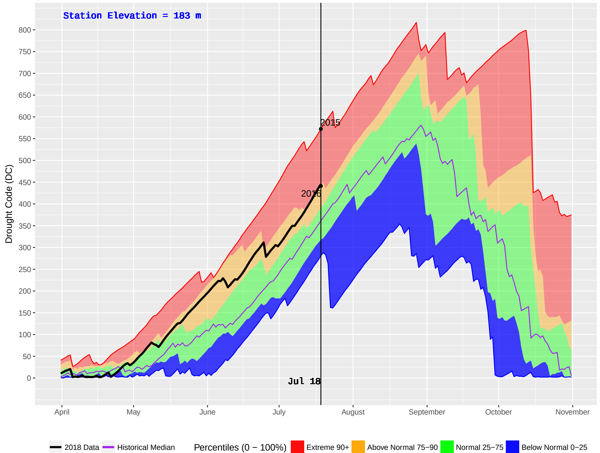
MESACHIE 2 (934) : Historical (2006–2016) and Current (2018) Daily Drought Code (DC)
