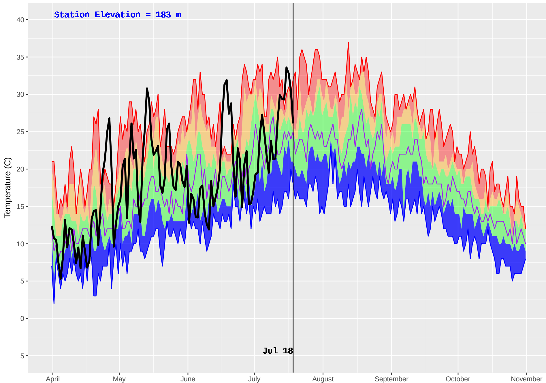
MESACHIE 2 (934) : Historical (2006–2016) and Current (2018) Daily Temperature
